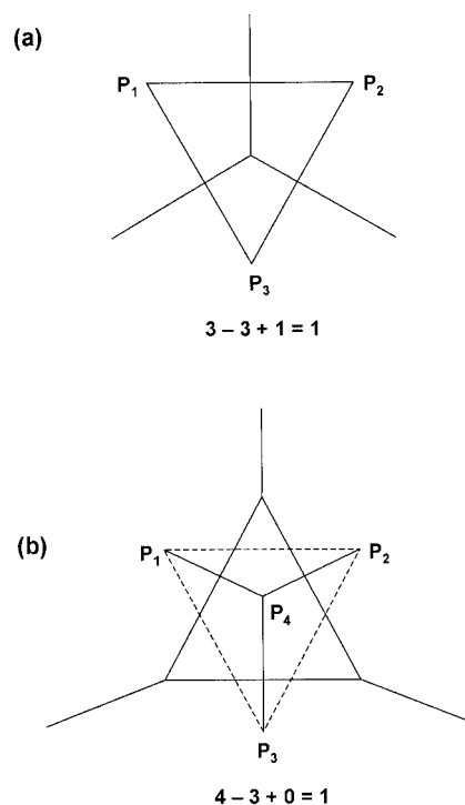
Figure 4. Examples of the Euler formula.
