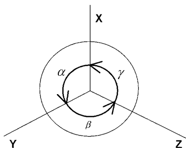
Figure A2. Structure of the nearest neighboring cells.
