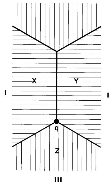
Figure A1. Cells prescribed to the vortex q on the sphere.
