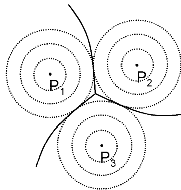
Figure 1. Organizing centers on the plane IR^2 .
